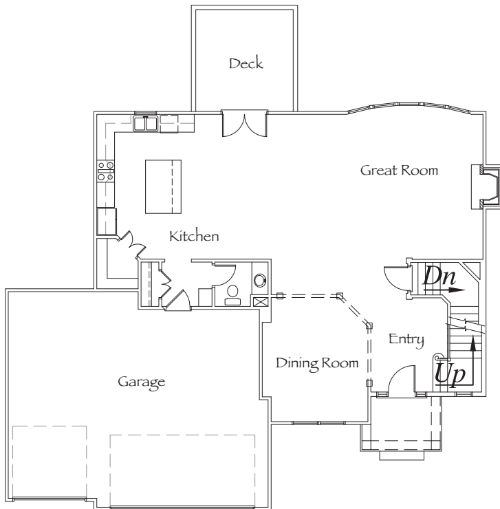
1st Floor Plan 1277 sq ft
