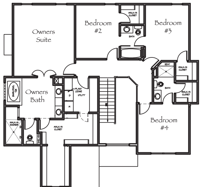
2nd Floor Plan 1435 sq ft
