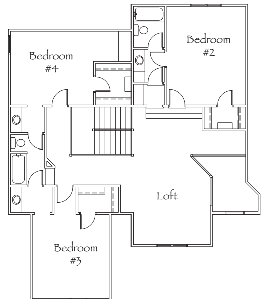
2nd Floor Plan 1401 sq ft
